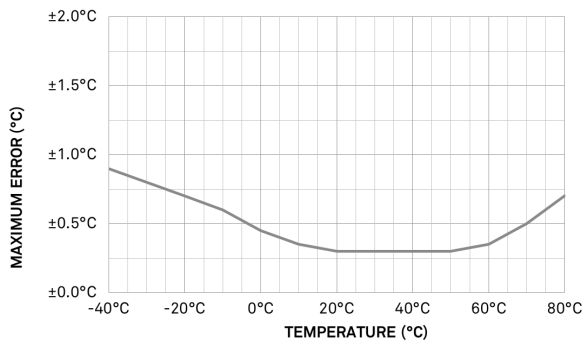
Figure 3 Temperature accuracy
